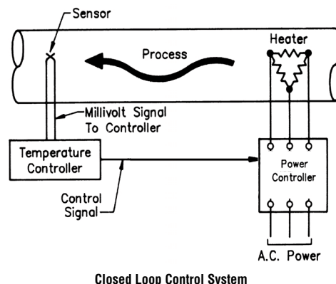
Closed Loop Control System
