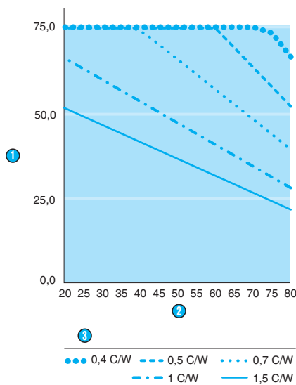
GN 75 AMP SSR (1200 & 600 V)
